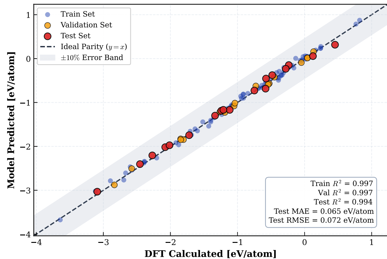
(b) Formation Energy ( E_f )
