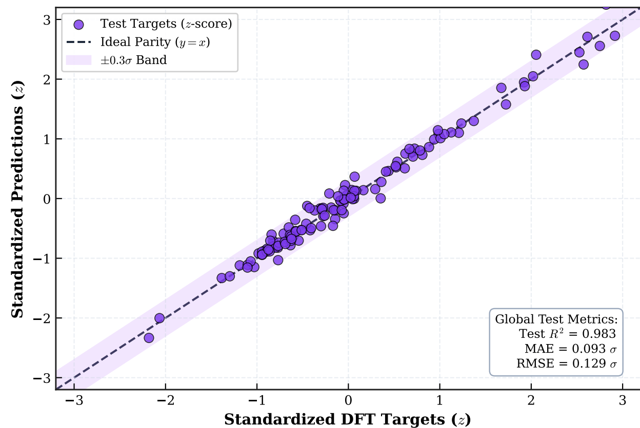
(h) Global Multi-Target Parity (Standardized)
