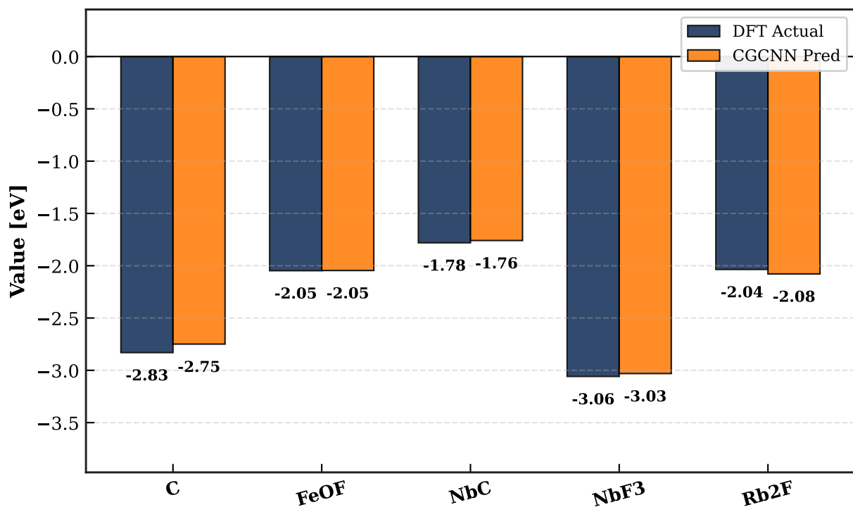
(g) Li Adsorption Energy ( E_{\text{ads}} )
