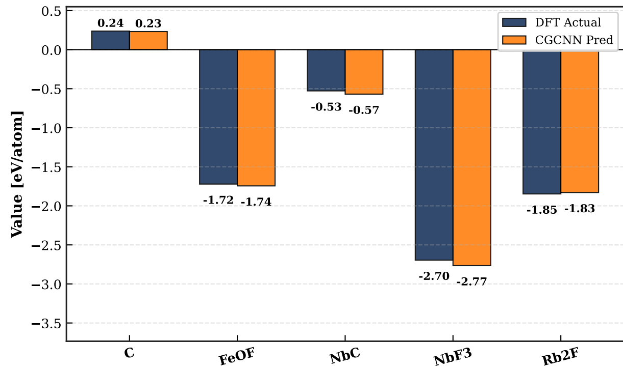
(b) Formation Energy ( E_f )
