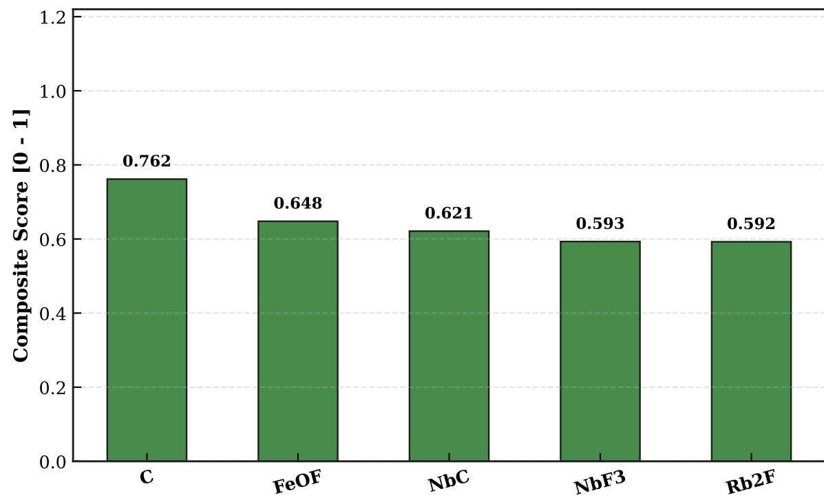
(h) Multi-Criteria Anode Screening Score
