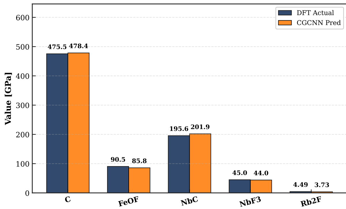
(e) Shear Modulus ( G )
