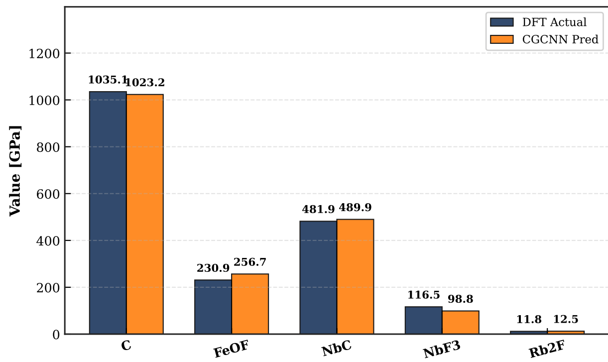
(f) Young's Modulus ( E )
