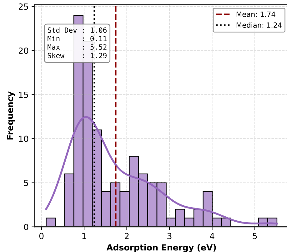
(e) Distribution of Adsorption Energy (eV)
