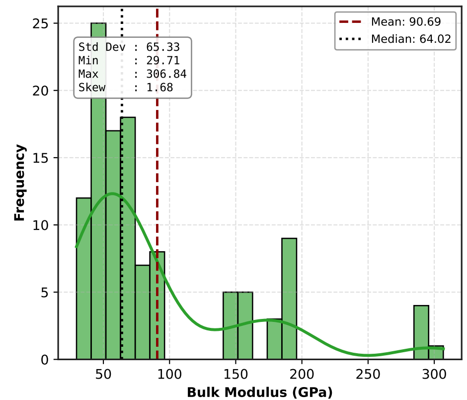
(c) Distribution of Bulk Modulus (GPa)
