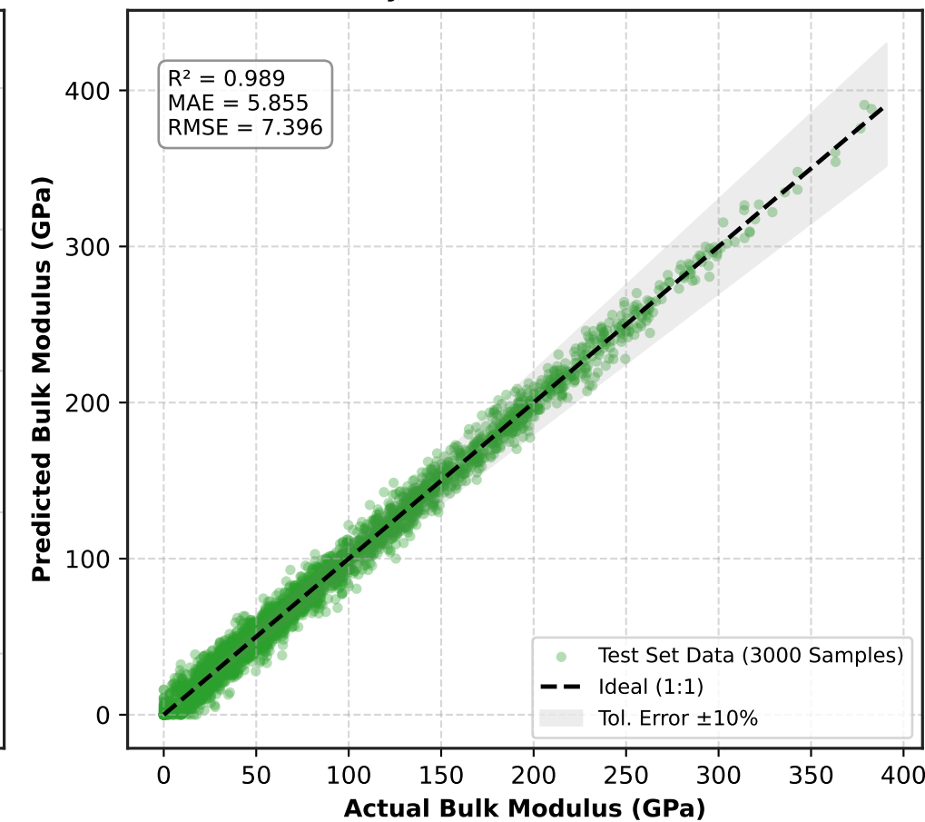
(c) Parity Plot: Bulk Modulus (GPa)
