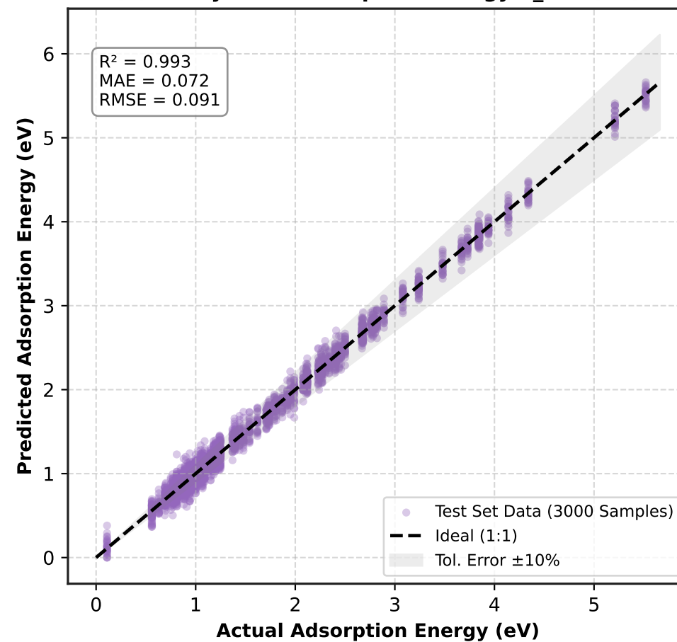
(e) Parity Plot: Adsorption Energy E_{ads} (eV)
