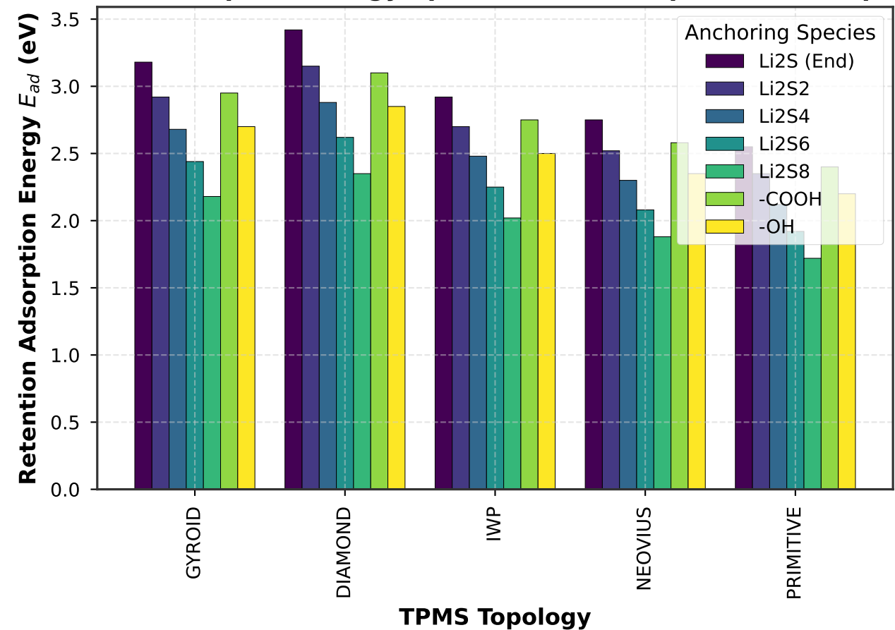
(b) Adsorption Energy Spectrum Across Species & Groups
