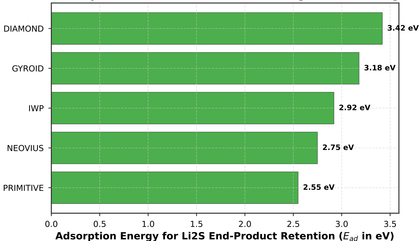
(a) Polysulfide End-Product (Li2S) Holding Power Ranking
