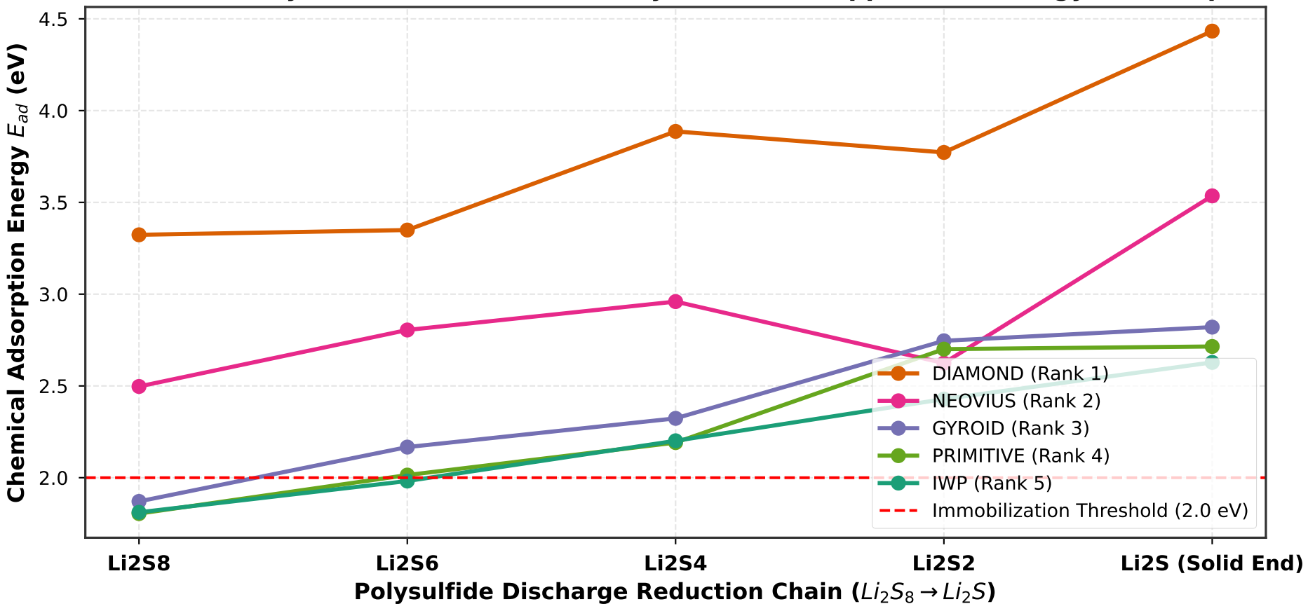
Chemical Polysulfide Reduction Pathway & Shuttle Suppression Energy Landscape
