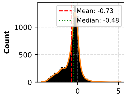
(c) Form. Energy (eV/atom)
