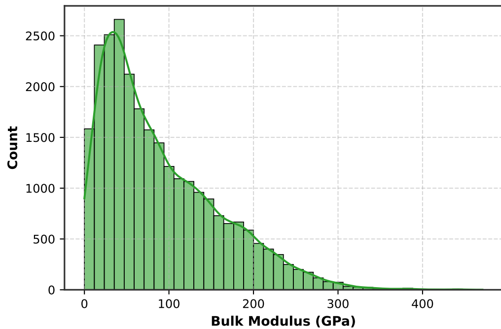
(c) Bulk Modulus (GPa) Distribution
