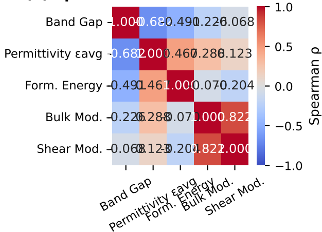
(b) Spearman Rank Correlation Matrix
