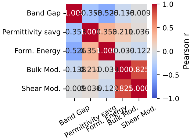
(a) Pearson Correlation Matrix
