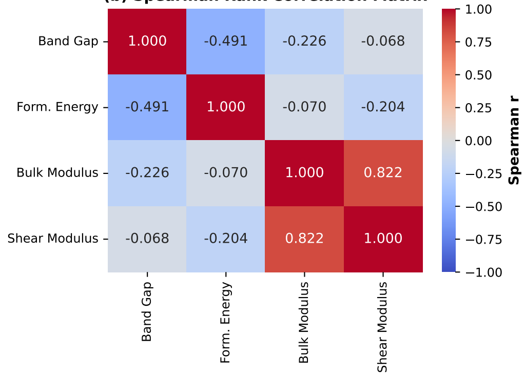
(b) Spearman Rank Correlation Matrix
