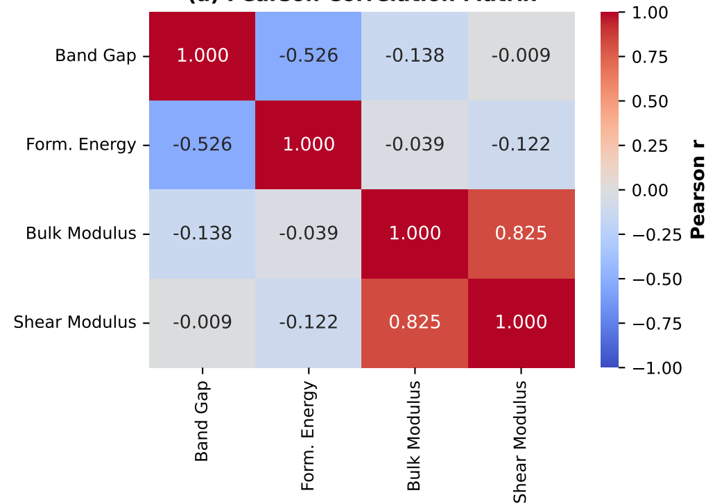
(a) Pearson Correlation Matrix
