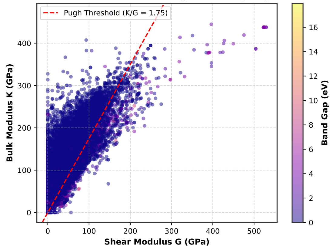
(b) Mechanical Moduli & Pugh's Ductility Map
