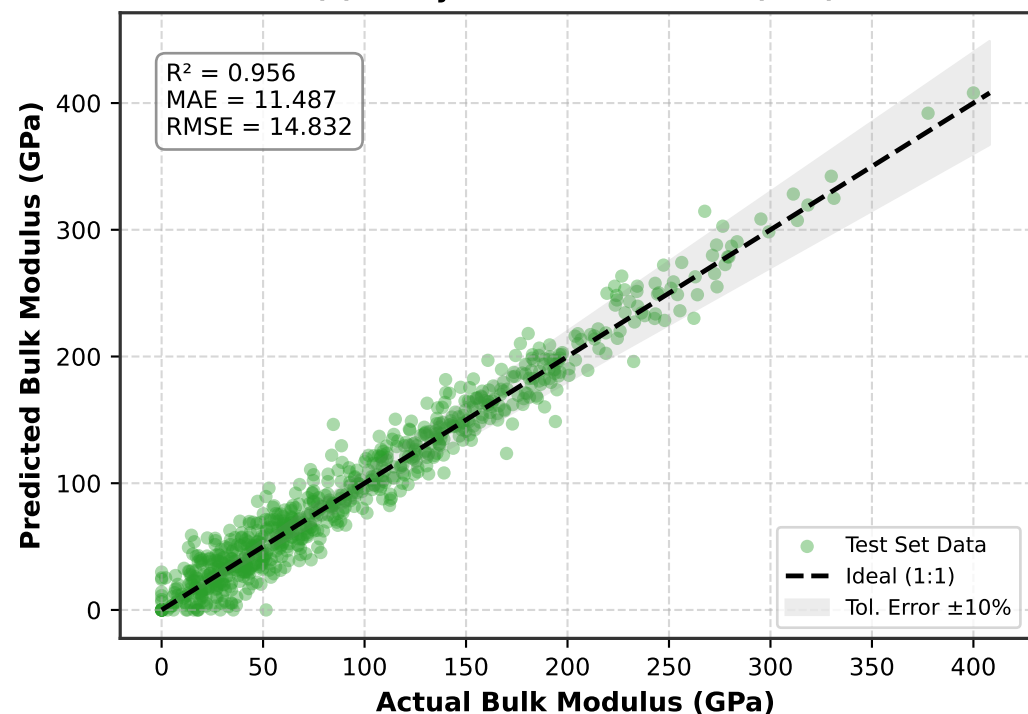
(c) Parity Plot: Bulk Modulus (GPa)
