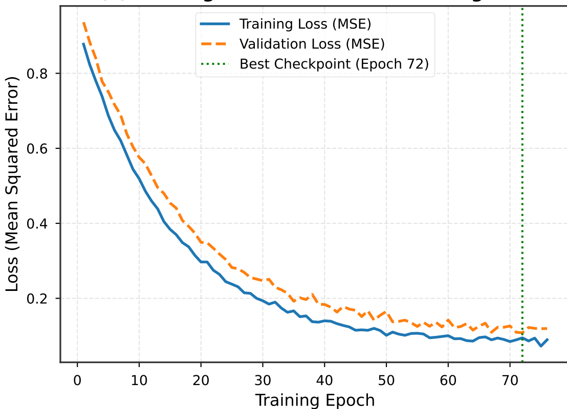
(a) Training & Validation Loss Convergence
