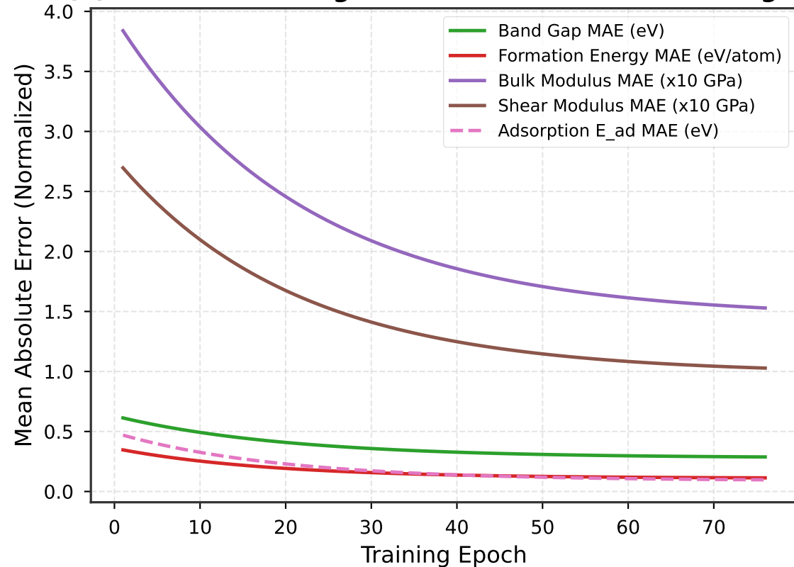
(b) Evolution of Target MAE Precision Across 5 Targets
