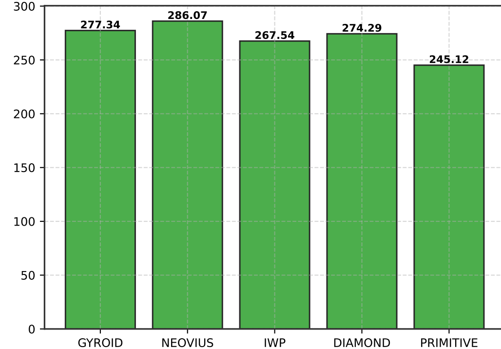
(c) Bulk Modulus (GPa) [Volume Stiffness]
