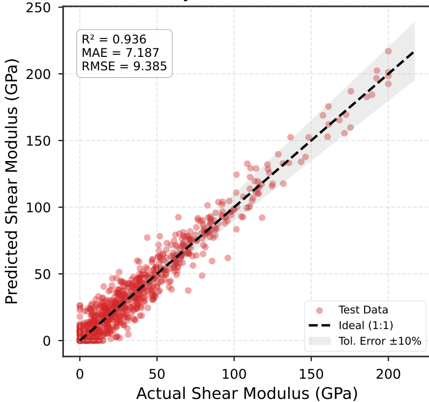
Parity Plot: Shear Modulus
