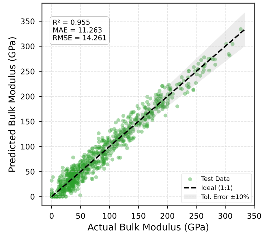
Parity Plot: Bulk Modulus
