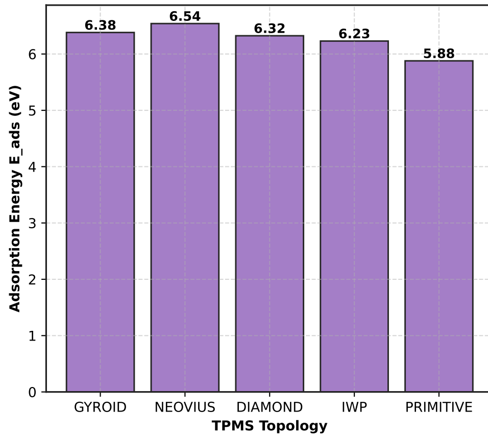
(e) Adsorption Energy E_{ads} (eV)
