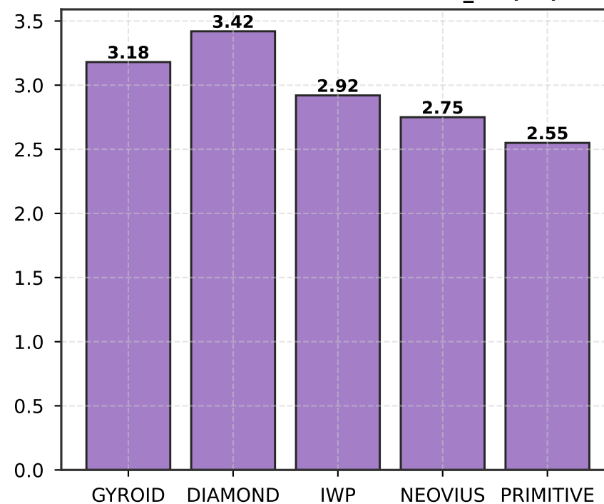
Li2S End-Product Retention E_{ad} (eV)
