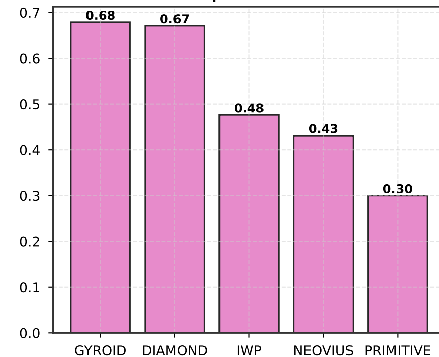
Li-S Composite Host Score
