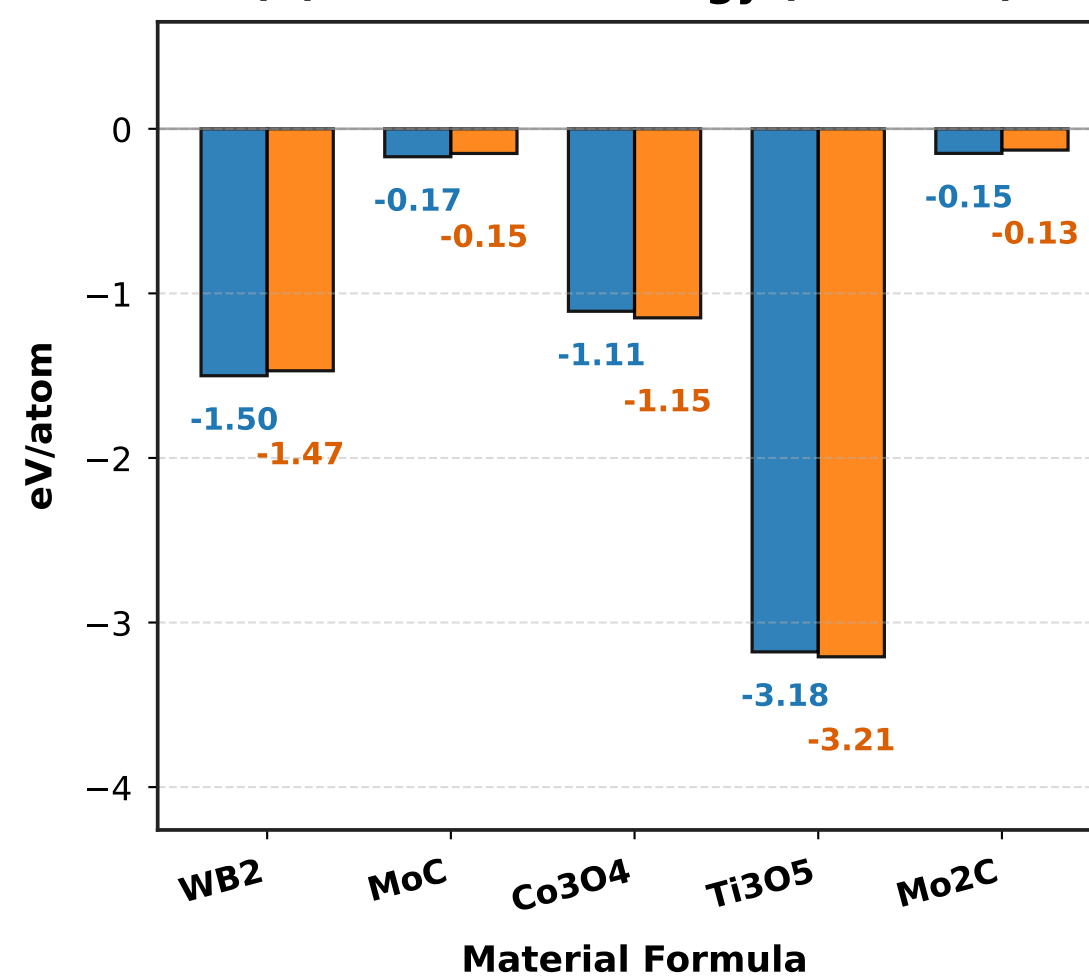
(b) Formation Energy (eV/atom)
