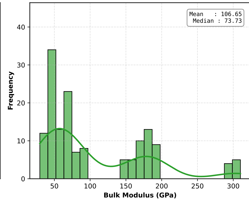
(c) Distribution of Bulk Modulus (GPa)
