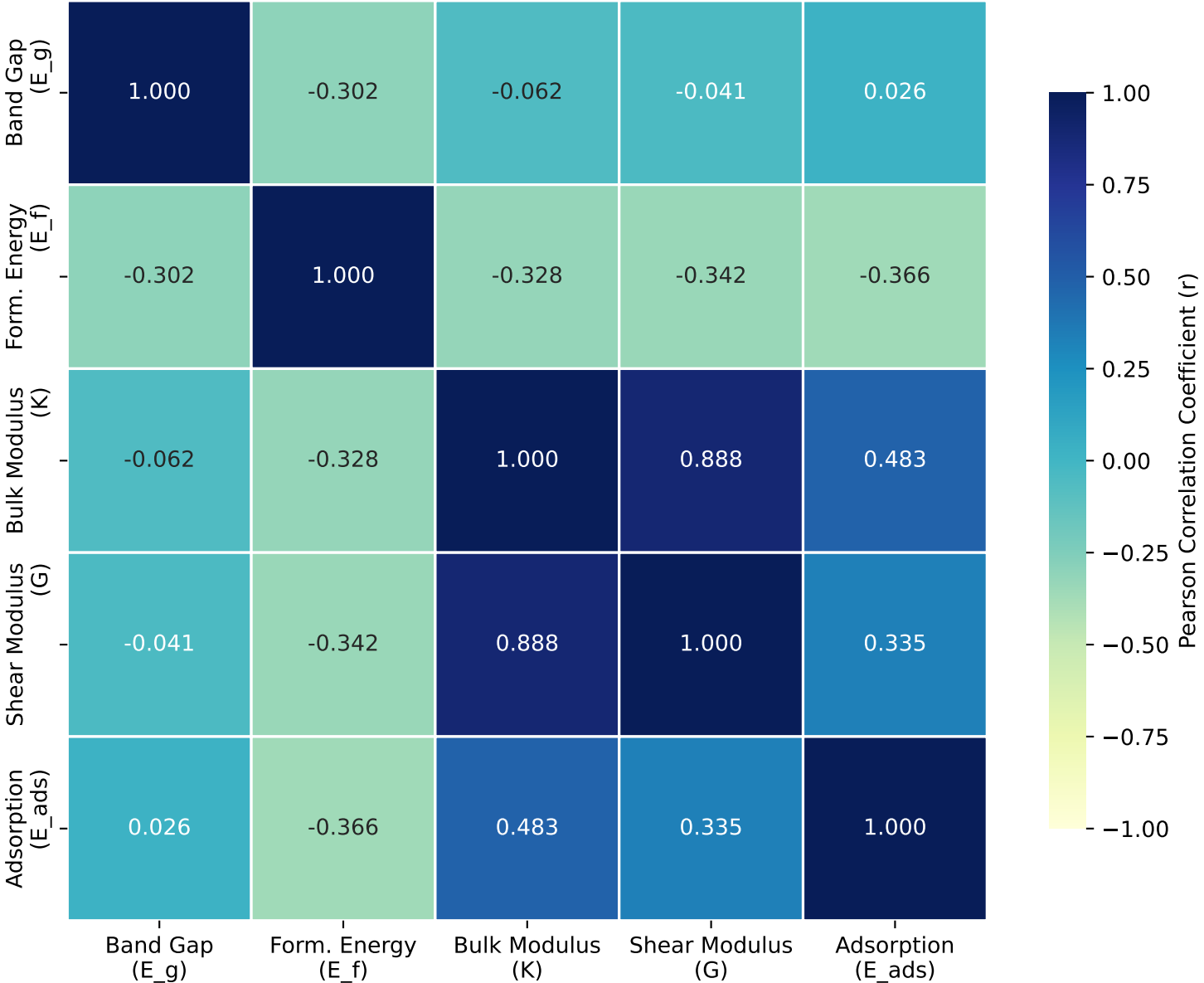
Inter-Property Linear Correlation Matrix across 5 Core Properties
