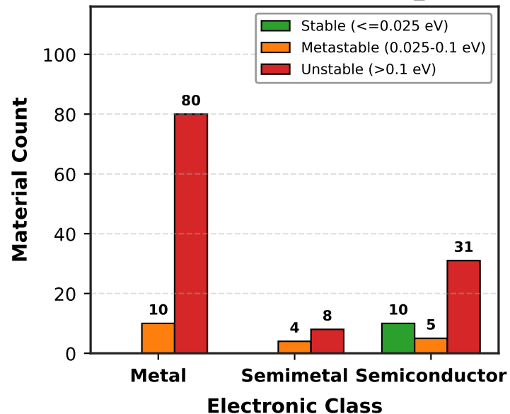
(b) Stability (by JARVIS E_hull)
