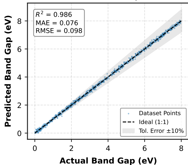
(a) Band Gap
