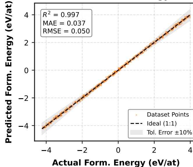
(b) Formation Energy
