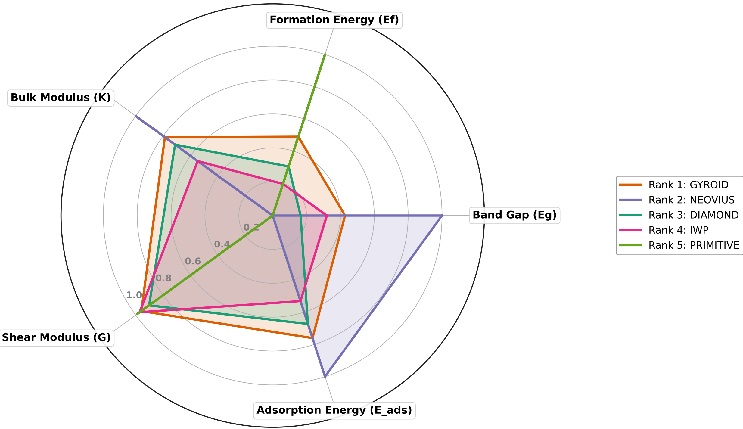
Holistic 5-Axis Performance Radar Map across 5 Core Physical Properties
