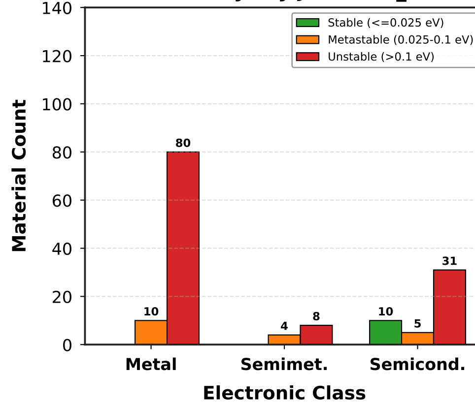
(b) Stability (by JARVIS E_hull)
