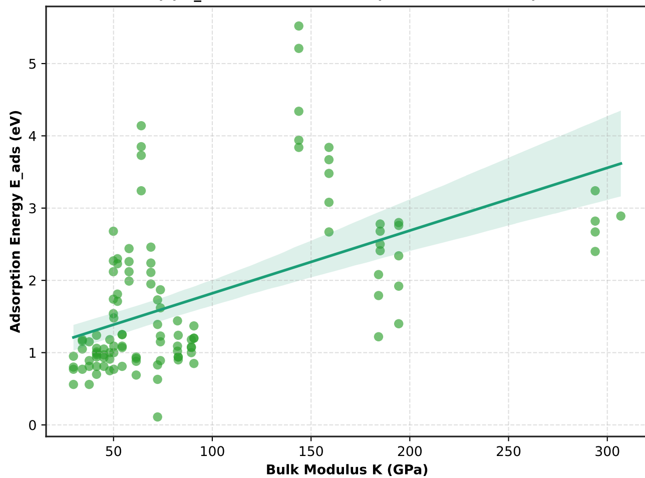
(c) E_{\text{ads}} vs Bulk Modulus (Pearson r = 0.533 )
