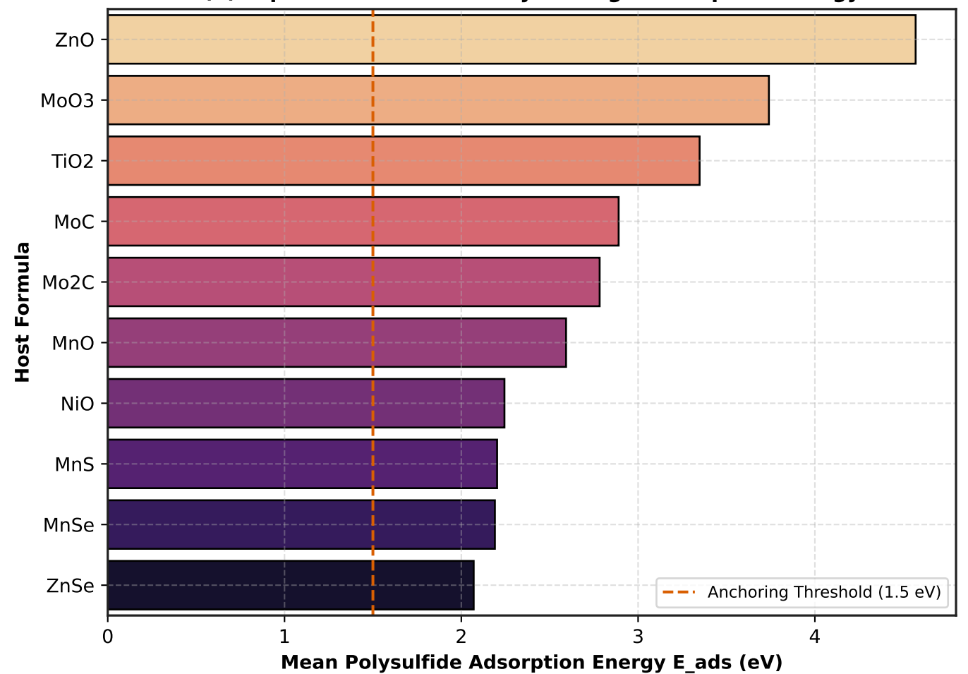
(d) Top 10 Host Materials by Average Adsorption Energy
