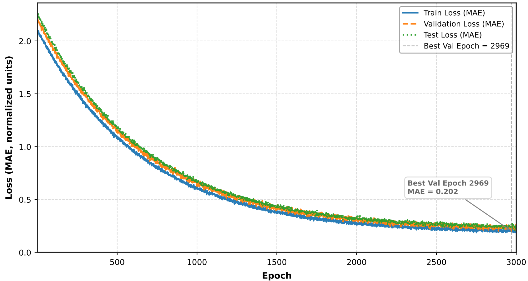
CGCNN Model Training, Validation, and Test Convergence Curves (3000 Epochs)
