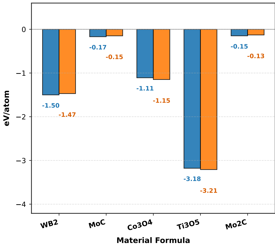
(b) Formation Energy (eV/atom)
