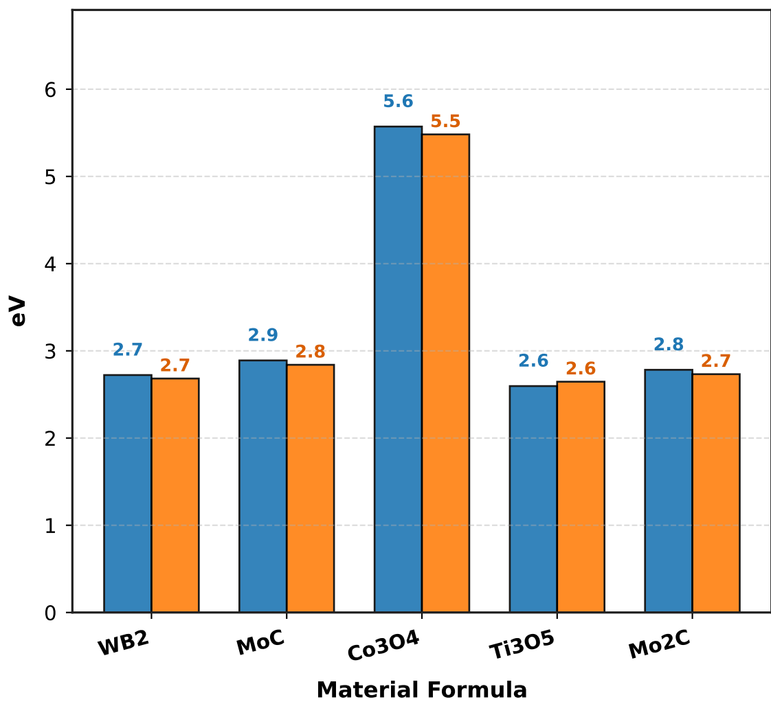
(e) Adsorption Energy (eV)
