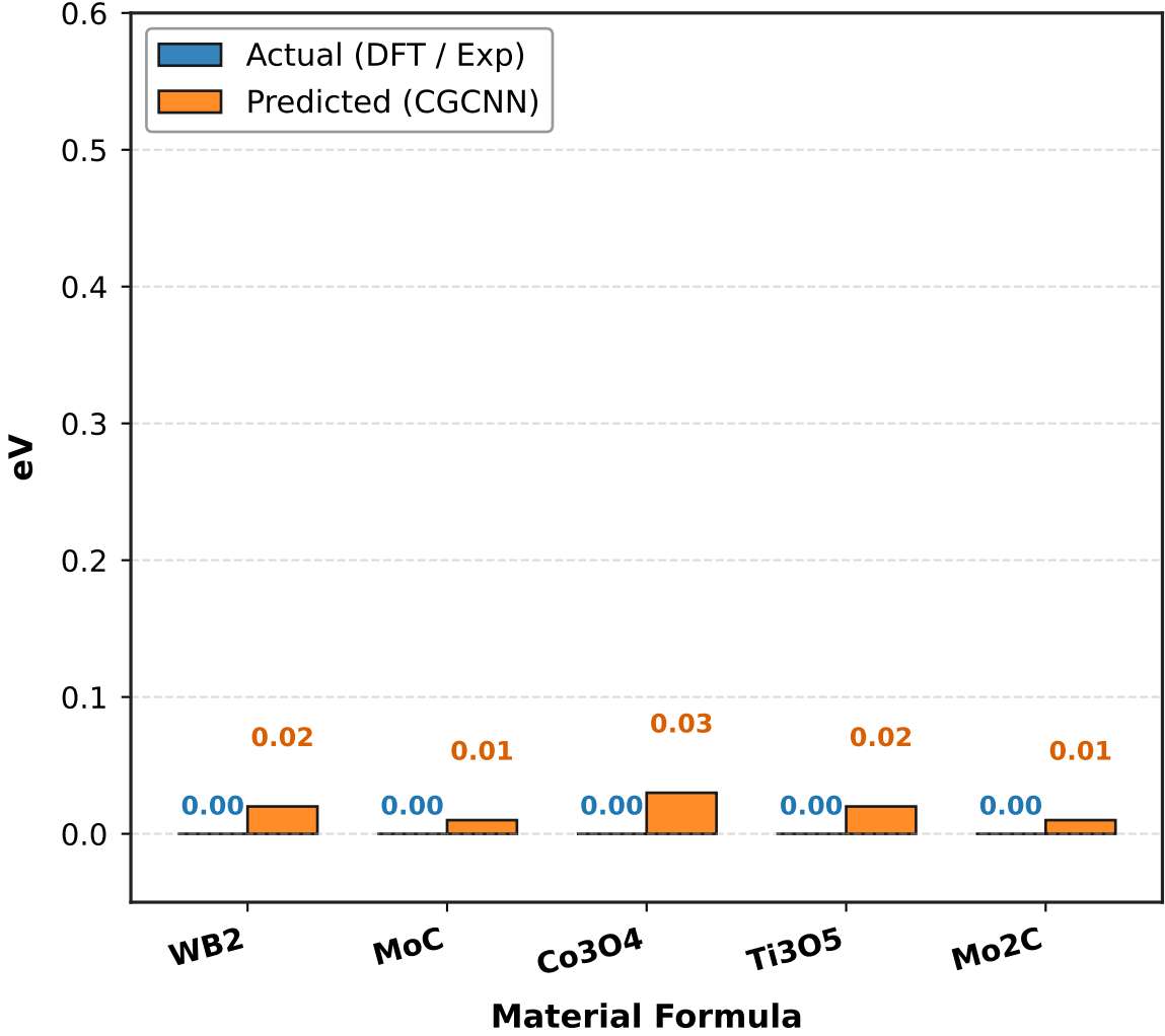
(a) Band Gap (eV)
