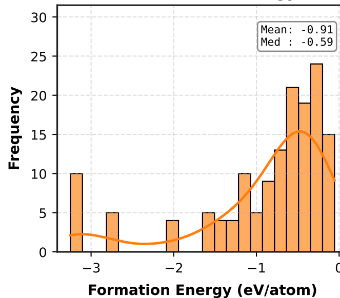
(b) Formation Energy
