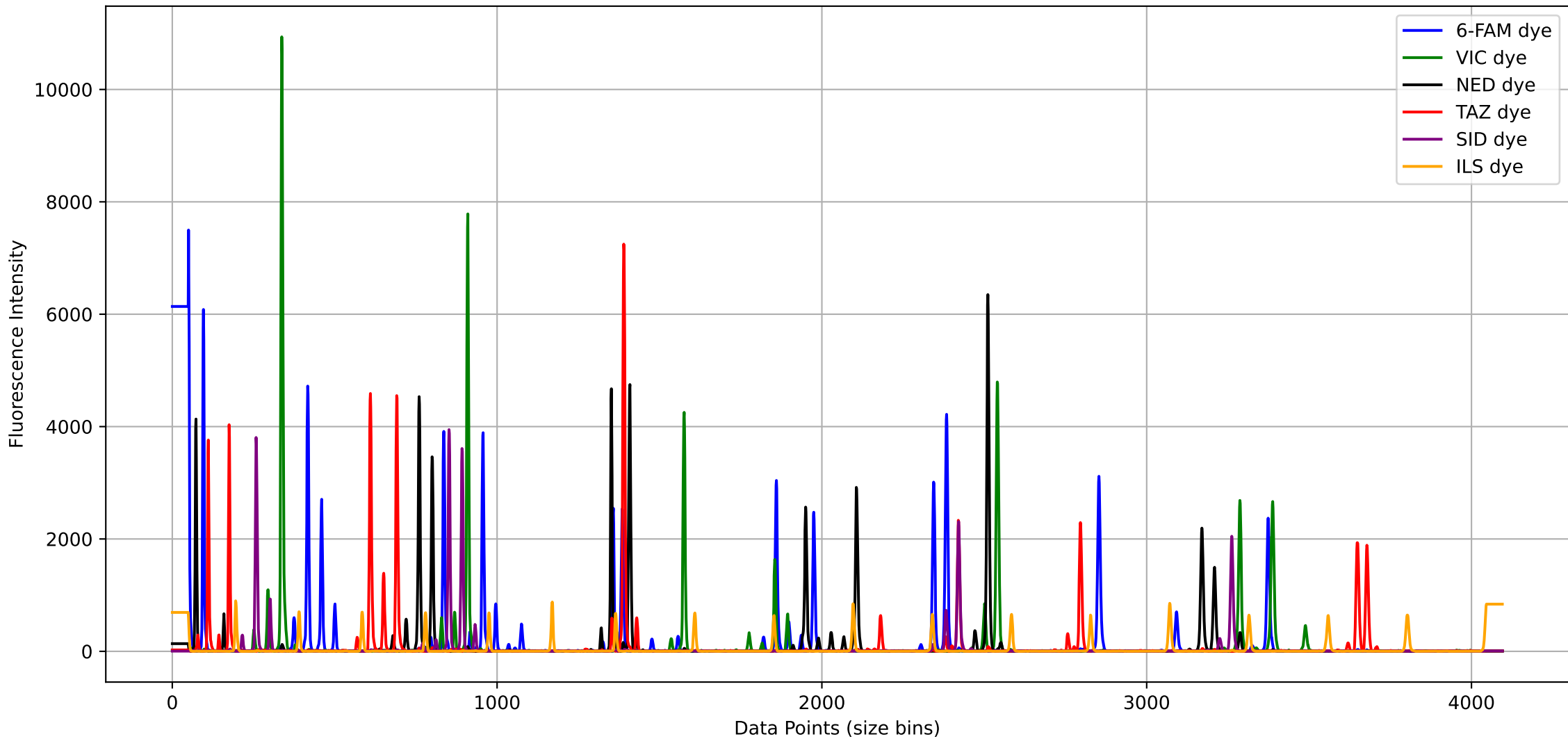
Electropherogram (EPG) Peak Signals Combined
