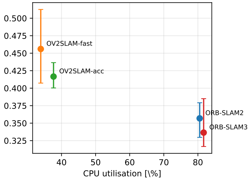
Accuracy versus cost (lower left dominates)
