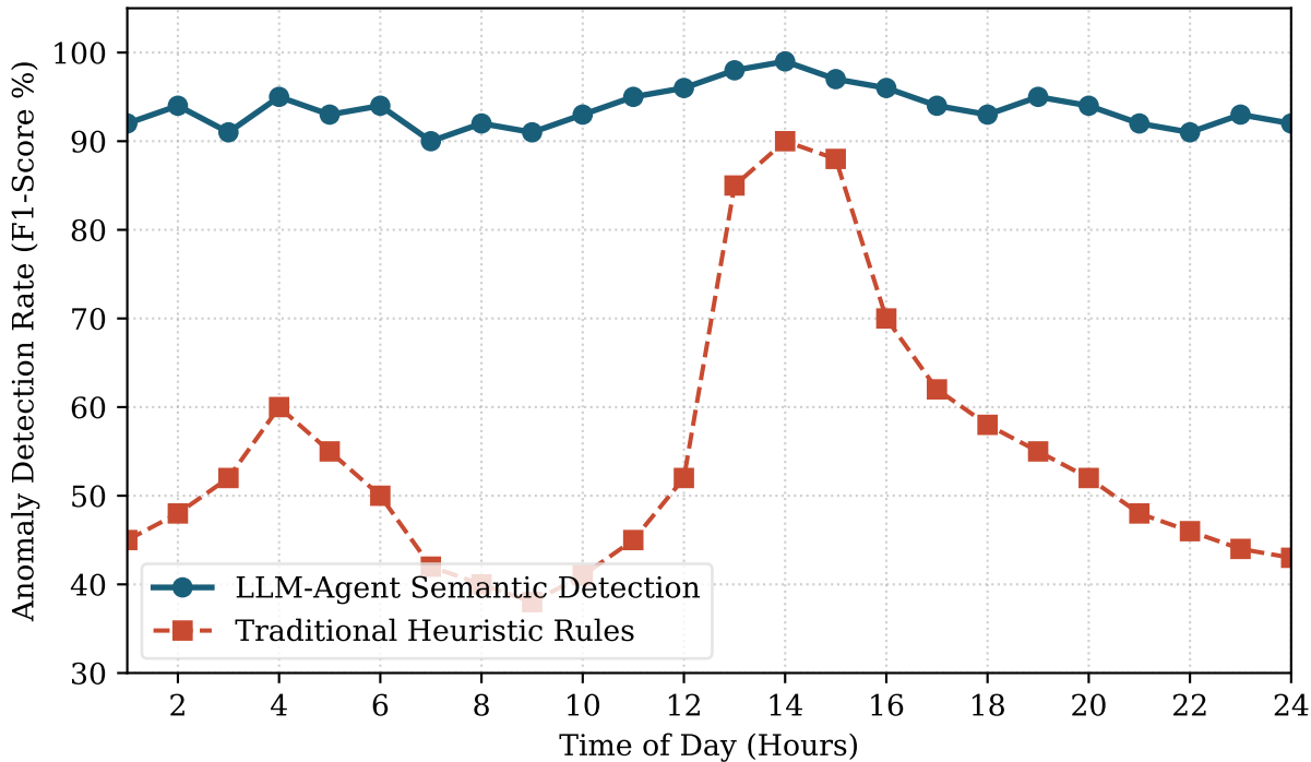
Network Anomalies Over Time: LLM vs. Heuristic Detection
