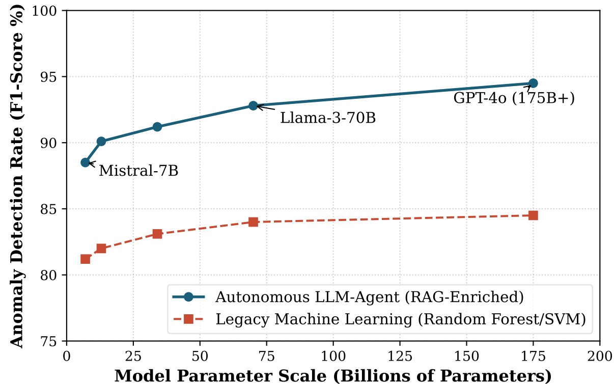
Detection Efficacy: LLM Agents vs. Legacy SOC ML Classifiers
