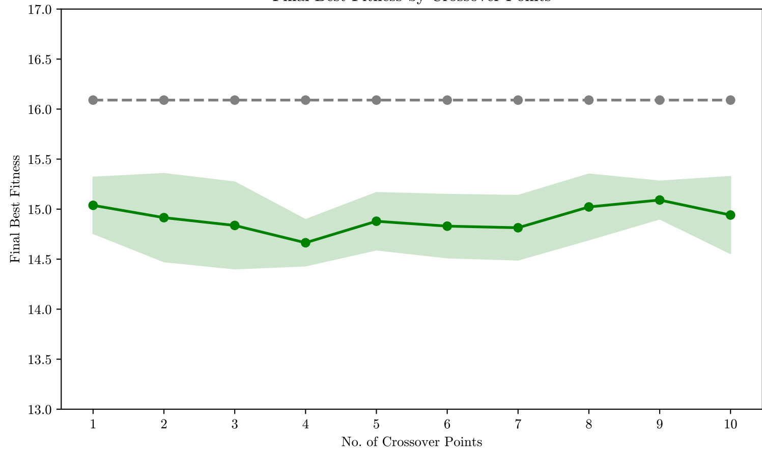
Final Best Fitness by Crossover Points
