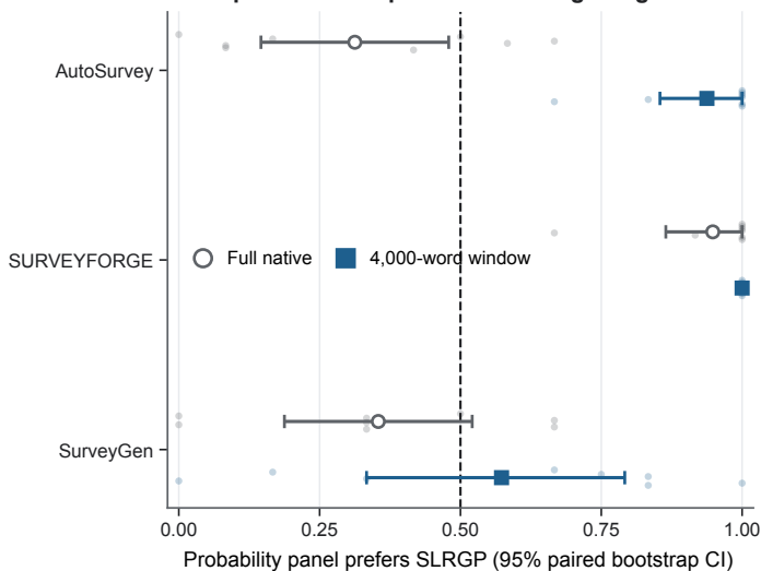
c Blind preference depends on reading budget
