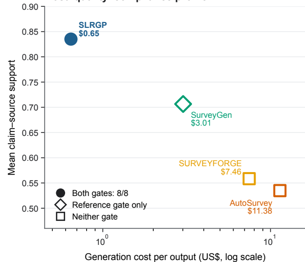
a Cost-quality-compliance profile
