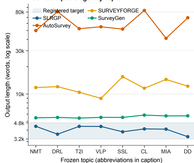
b Native output length by topic
