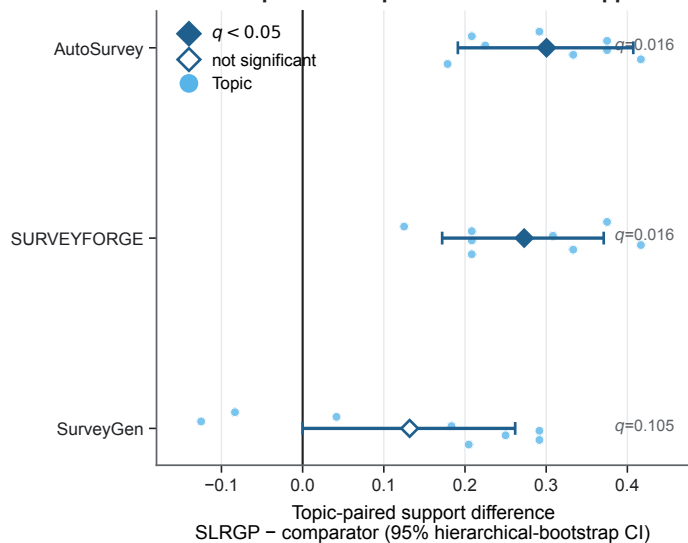
d SLRGP improves sampled claim-source support
