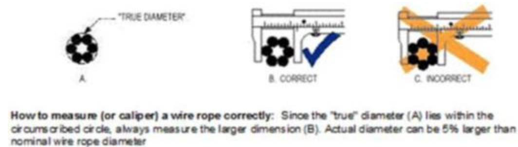
Figure 12.9. Correct and Incorrect Way to Measure Wire Rope. (Note: Always read the widest diameter.)
