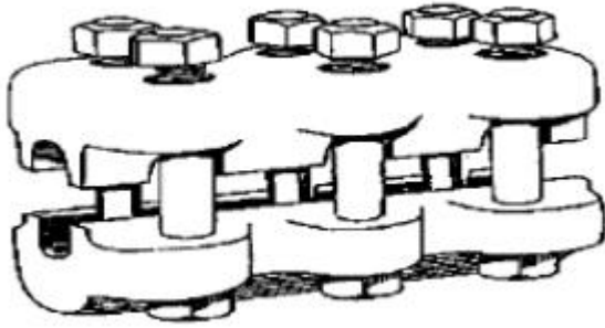
Figure 12.7. Joining Wire Ropes.
