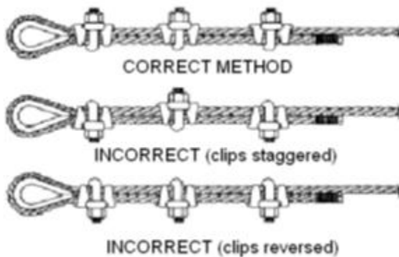
Figure 12.4. Right and Wrong Way of Using Cable Clips.
