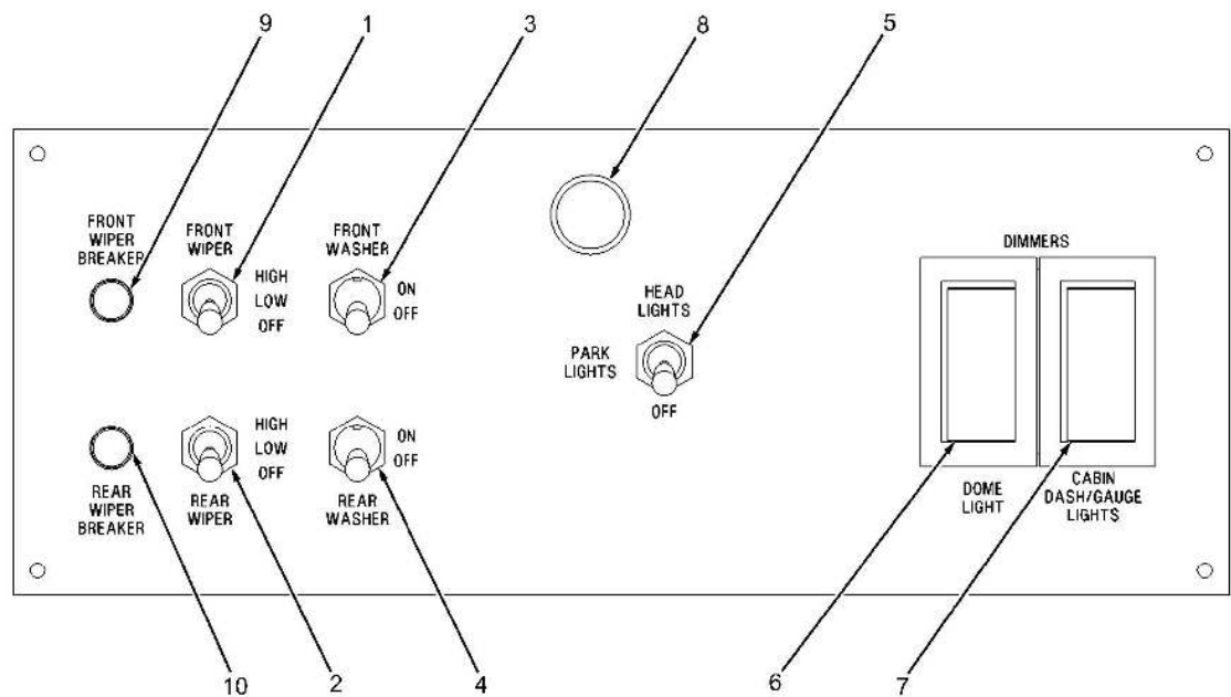
Figure 2-3. Wiper Panel
