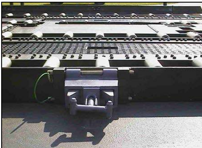
Figure 5.13. Pallet Restraint.
