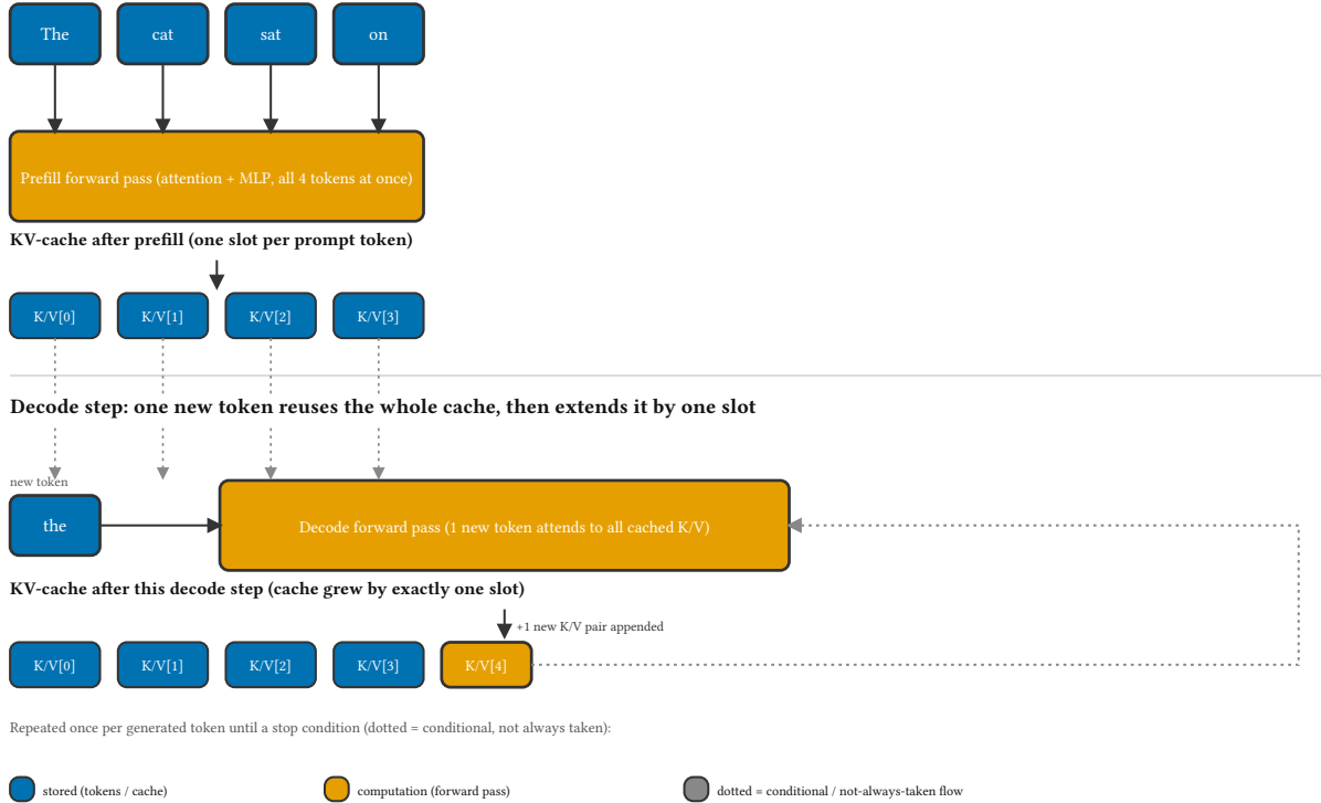
Figure 4: Prefill builds the whole cache from the prompt in one pass; each decode step afterward reads the entire cache but appends exactly one new K/V slot to it. This figure is reused as-is from the project’s existing KV-cache demonstration – the mechanics don’t change between this chapter’s introduction of the idea and Chapter 3’s deeper treatment of it.
