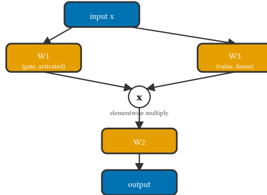
Gated MLP / SwiGLU (three matrices)
