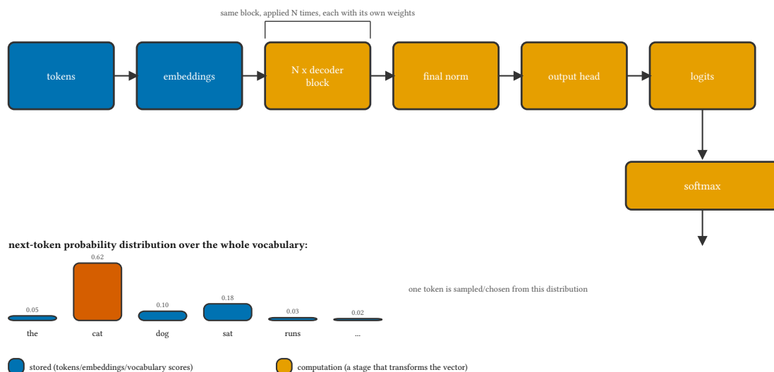
Figure 1: Tokens become vectors, the same block repeats N times with its own weights at each repetition, and only the final softmax turns a vector back into a probability distribution over the vocabulary – nothing “decides” the next token before that last step.
