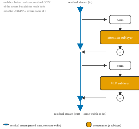
Figure 2: One block, showing the residual stream as the vertical bar and the two sublayers branching off it. Notice the stream’s width never changes – only what gets added to it does.
