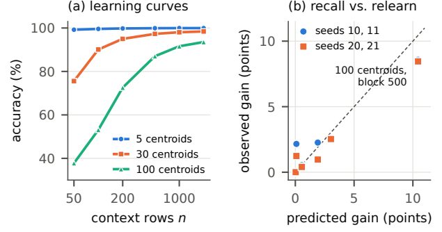
Figure 2. (a) Learning curves of the grid concepts with TabPFN v2, measured before the grid streams were run. (b) Gain of memory over reset per grid cell: predicted from these curves by Theorem 1 against observed, for the fast level on seeds 10 and 11 and for MICE on seeds 20 and 21; the dashed line is equality.
