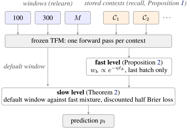
Figure 1. MICE for one batch. Windows and stored contexts are in-context experts of the same frozen TFM. The fast level mixes all experts from their losses on the last labelled batch; the slow level mixes the result with the default window. Each component is governed by one result of Section 3.
