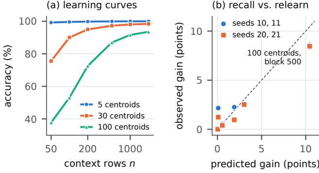
Fig. 2. (a) Learning curves of the grid concepts with TabPFN v2, measured before the grid streams were run. (b) Gain of memory over reset per cell: predicted from these curves (registered values, see Section 5.1) against observed, for the fast level on seeds 10 and 11 and for MICE on seeds 20 and 21; the dashed line is equality.
