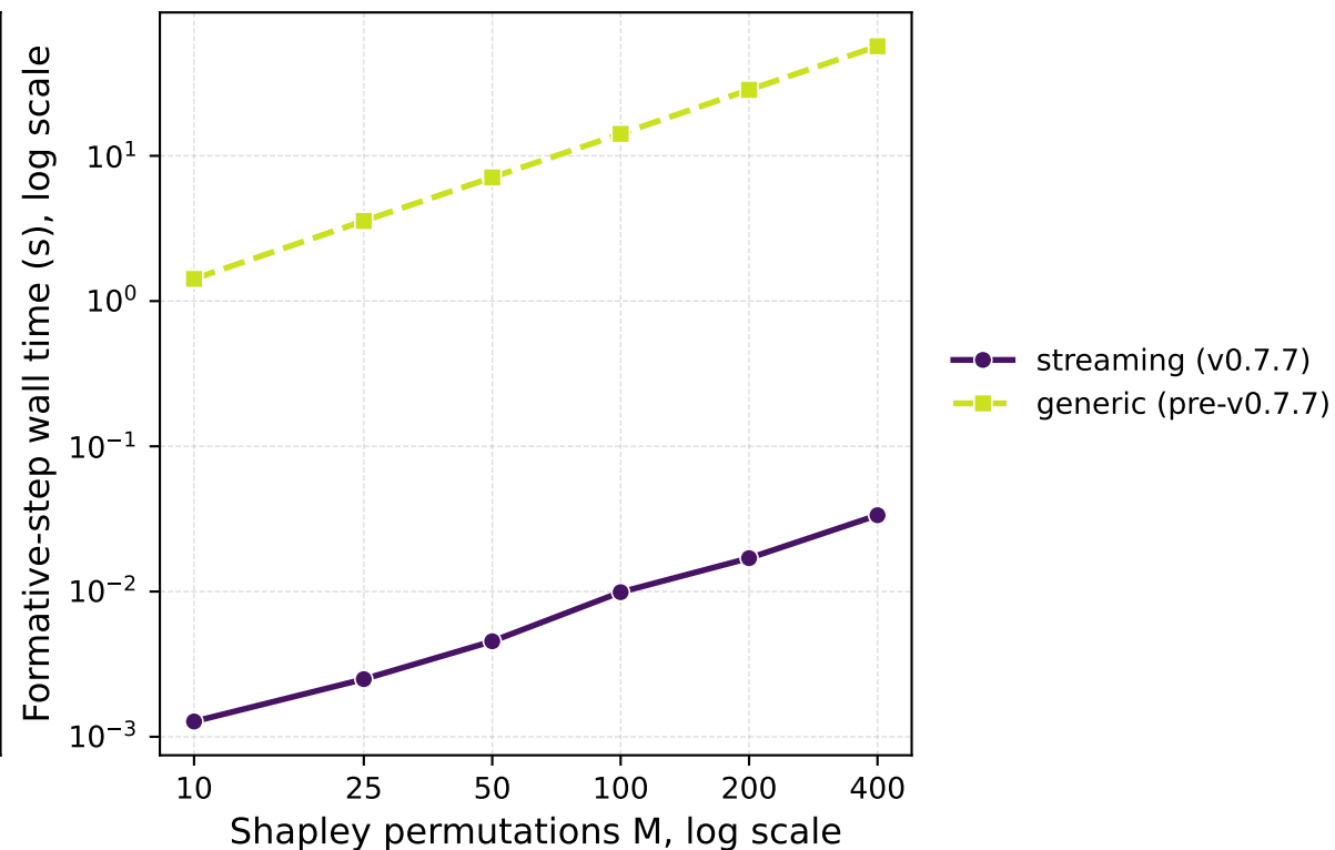
(c) Runtime vs M ( n=1000 , d=8 )
