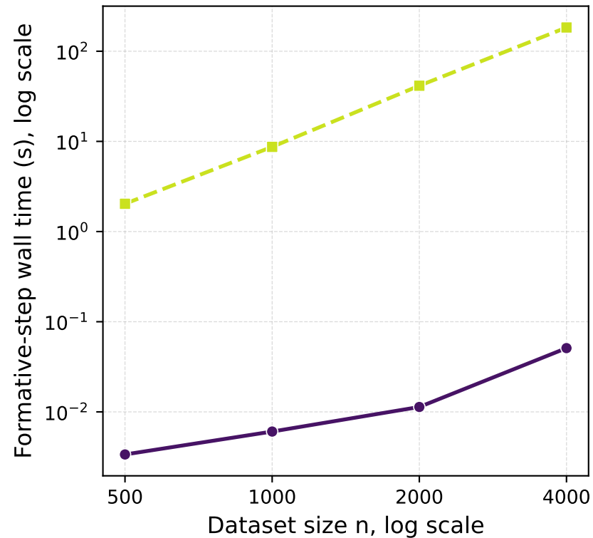
(a) Runtime vs n ( d=8 , M=50 )
