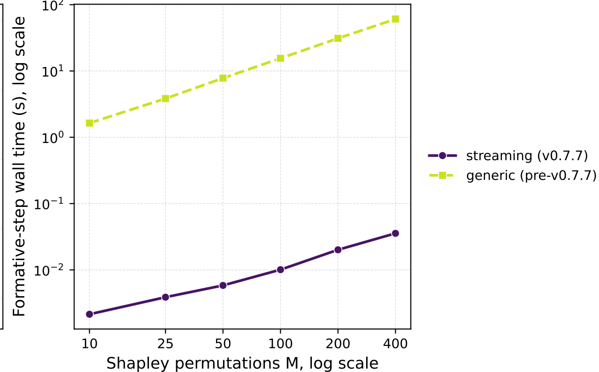
(c) Runtime vs M ( n=1000 , d=8 )
