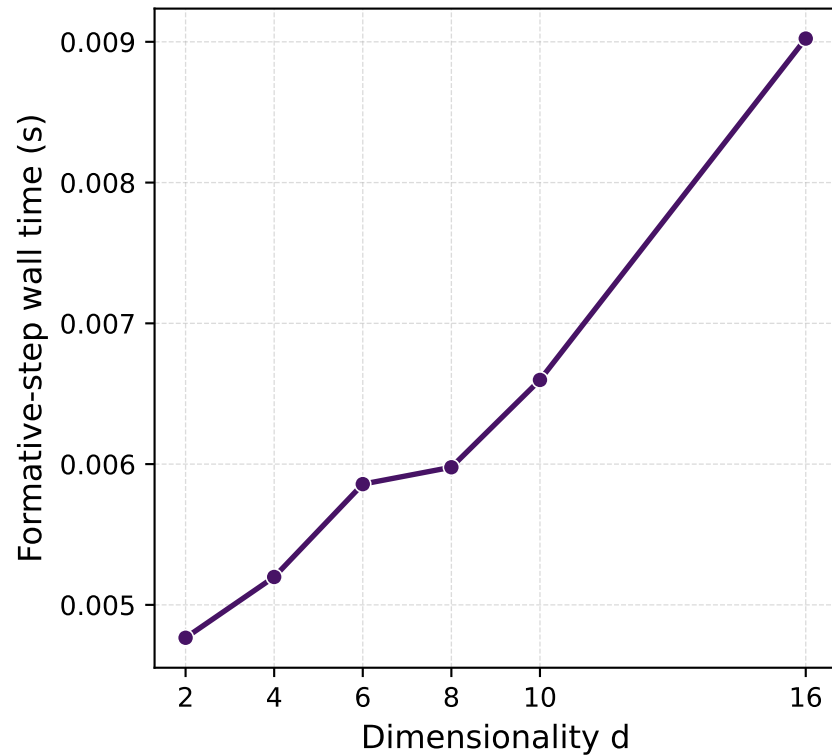
(b) Runtime vs d ( n=1000 , M=50 )
