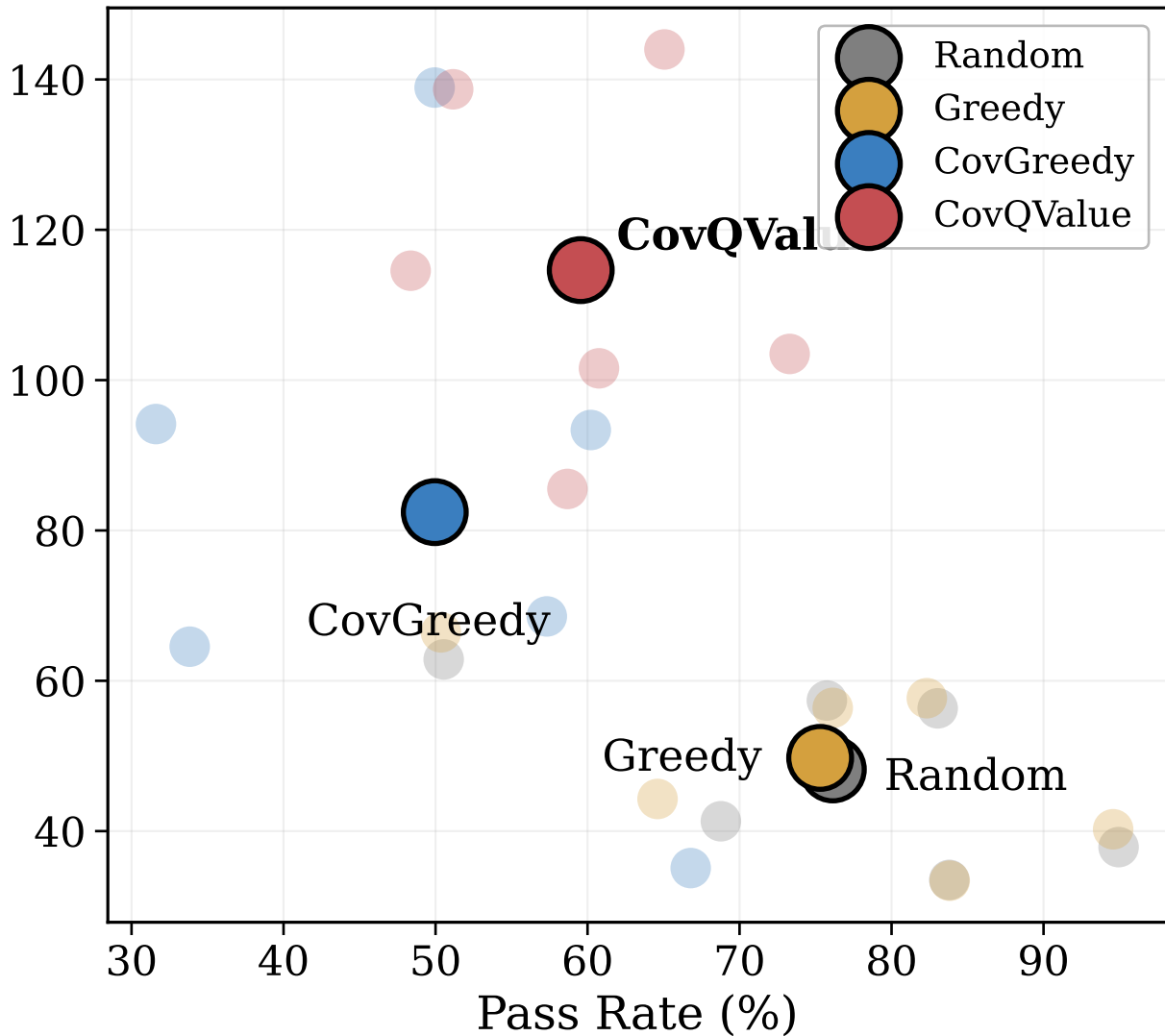
Mean Branch Coverage
