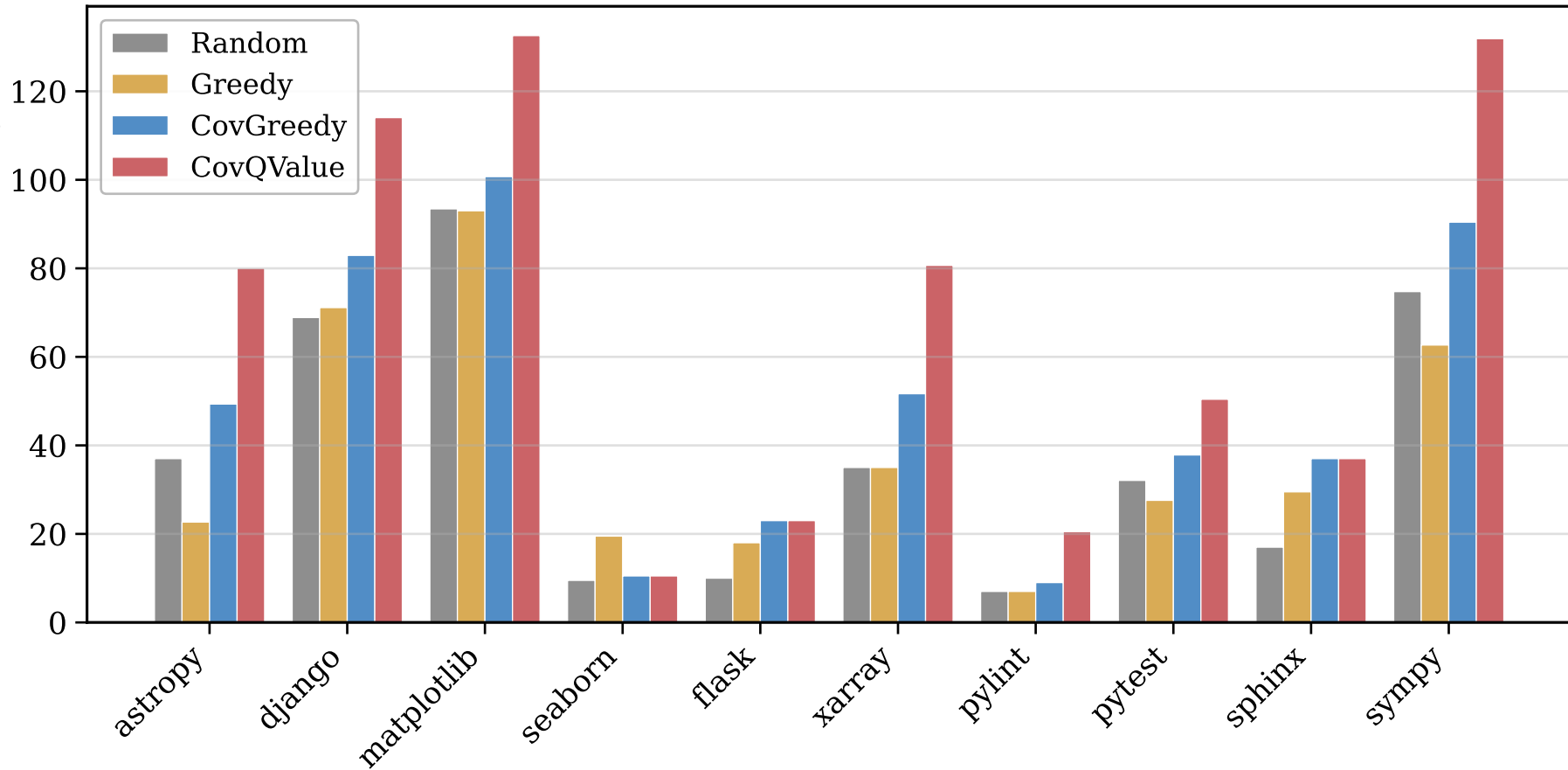
Mean Branch Coverage
