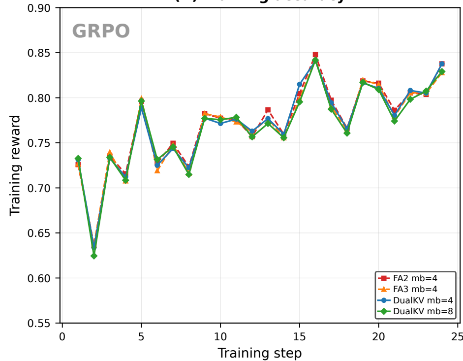
(A) Training accuracy
