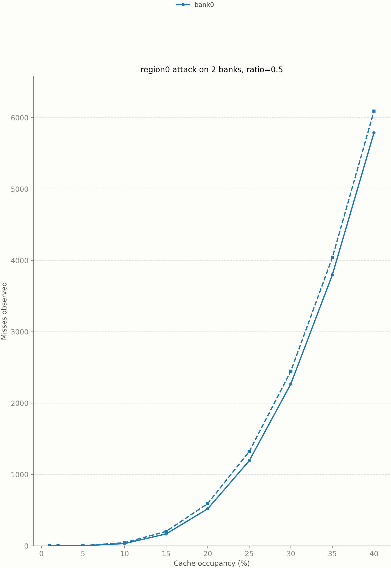
normal cache - 2-bank region0 ratio 0p5 (solid=bit0, dashed=bit1)
