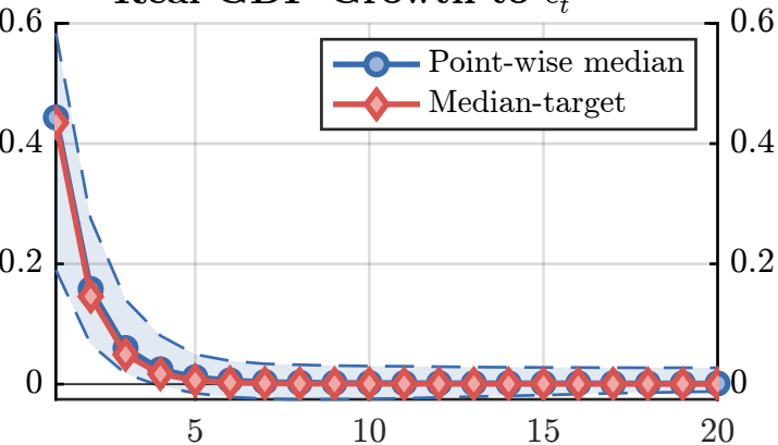
Real GDP Growth to \epsilon_t^{\text{Demand}}
