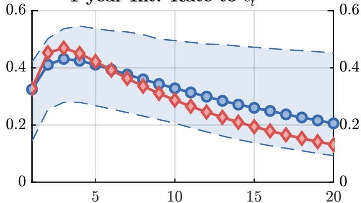
1-year Int. Rate to \epsilon_t^{\text{Demand}}
