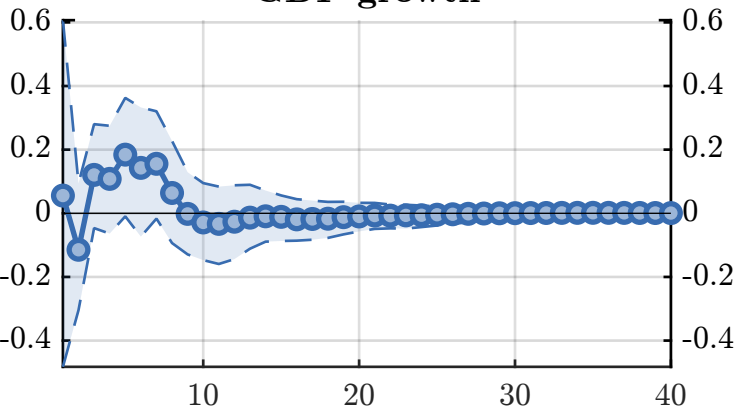
GDP growth
