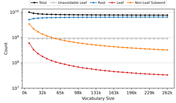
Figure 13: Validation counts for ToaST with 700k split trees by Leaf (single byte tokens), Unavoidable Leaf (single-byte pretokens), Non-Leaf Subword, and Root nodes (single token for pretoken), on a log scale.
