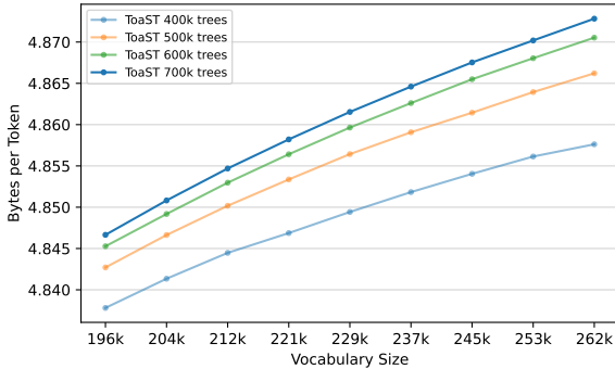
Figure 12: Validation bytes per token of ToaST, zoomed in for larger vocabulary sizes.
