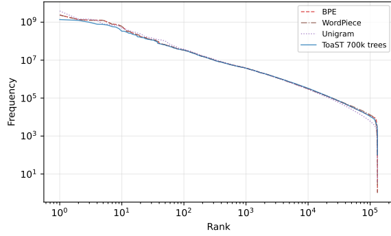
Figure 16: Zipf plot of the validation token frequency vs. token rank for ToaST, BPE, WordPiece, and UnigramLM with 128k vocabularies.
