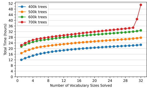
Figure 10: Cumulative total time to set up and solve the model, as a function of the number of vocabulary sizes computed.
