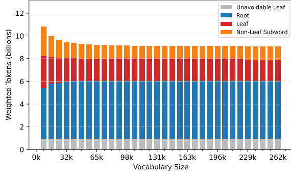
Figure 15: Token categories for UnigramLM, using the same categories as ToaST.
