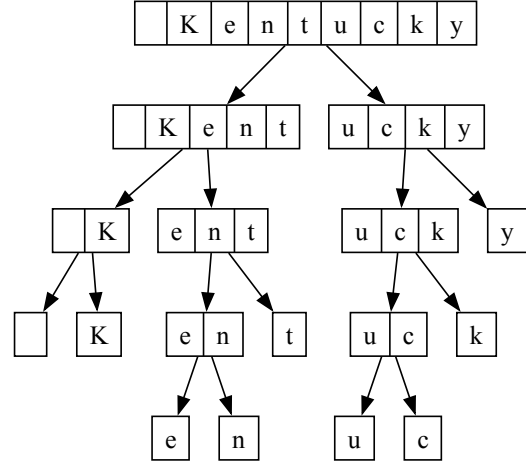
Figure 1: Example split tree for ‘Kentucky’.
