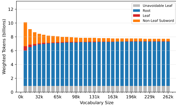
Figure 6: Stacked validation token categories for ToaST with 700k split trees by Leaf (single byte tokens), Unavoidable Leaf (single byte pretokens), Non-Leaf Subword, and Root nodes (single token for pretoken).
