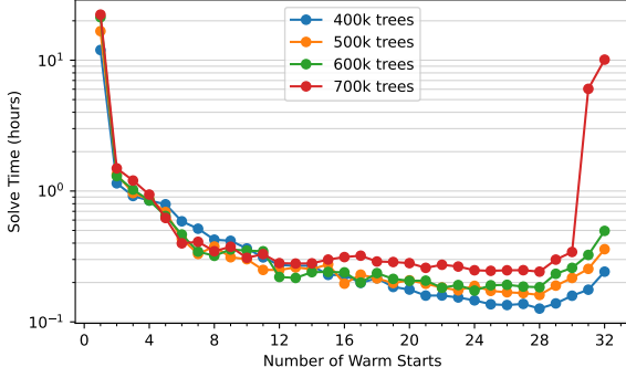
Figure 11: Individual timing of each resolve step, with the same setup as Figure 10, with a log scale on the y -axis solve time. Set up time is included in the first point.
