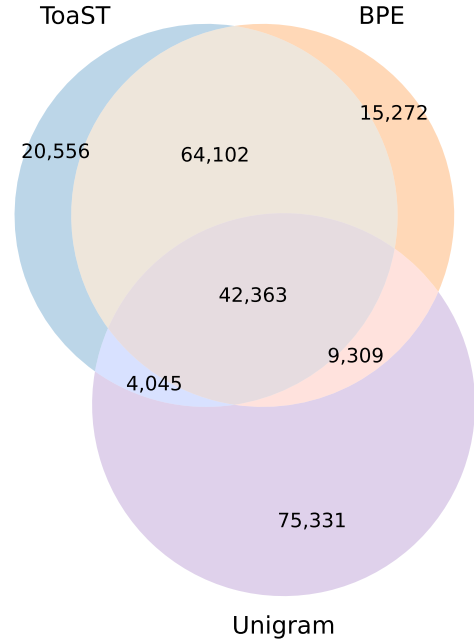
Figure 18: Venn diagram of overlap in the tokens used in the tokenization of the validation data, with a 128k vocabulary.
