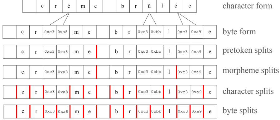
Figure 9: Example split hierarchy of pretokens \succ morphemes \succ characters \succ bytes for crème brûlée .
