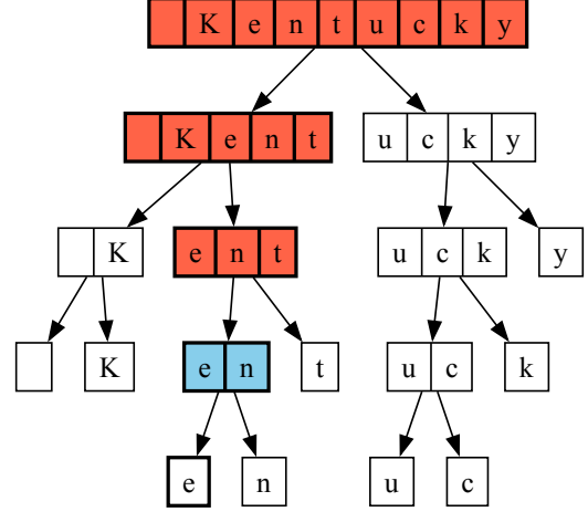
Figure 3: A node (blue) appears in the tokenization when it is in the vocabulary and none of its ancestors (red) are in the vocabulary. An example path from leaf node e to the root is also shown with a heavier black outline.
