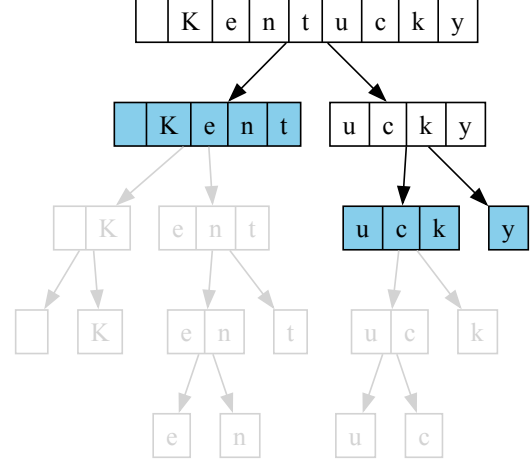
Figure 2: Example tokenization, with white tokens not in the vocabulary, used tokens (in the vocabulary) in blue, and nodes never reached in the recursive descent in light gray.
