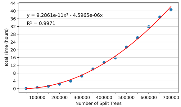
Figure 4: Total training time as a function of the number of split trees. In these runs the vocabulary size m is set to half the number of split trees.
