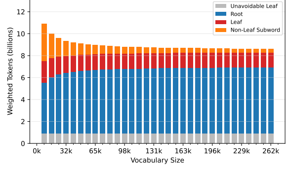
Figure 7: Validation token categories for BPE. Using the same categories as ToaST in Figure 6.
