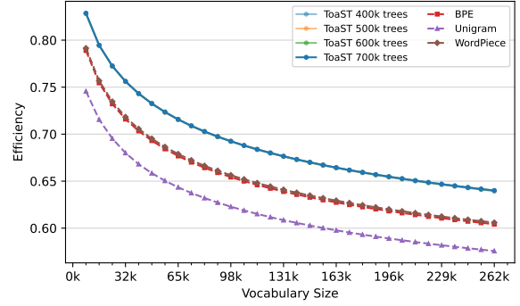
Figure 17: Validation Shannon efficiency ( \alpha = 1 ).
