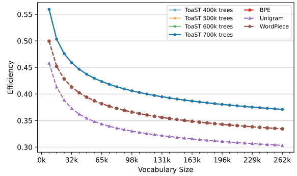
Figure 8: Validation Rényi efficiency ( \alpha = 2.5 ) for ToaST and several baselines as a function of vocabulary size. Higher is better, indicating a more uniform token distribution. The four ToaST series are very similar to each other, as are BPE and WordPiece.
