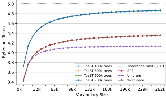
Figure 5: Validation data bytes per token for ToaST and several baselines, as a function of vocabulary size. Without the use of supermerges (Liu et al., 2025; Schmidt et al., 2025, 2026) there is an upper bound in which each pretoken is a single token, which is shown as a dotted line at 5.01 for the validation data.
