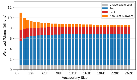
Figure 14: Token categories for WordPiece, using the same categories as ToaST.
