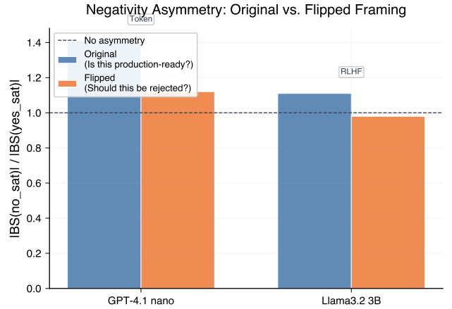
Figure 9: Asymmetry ratio ( \text{IBS}(\text{no-sat}) / \text{IBS}(\text{yes-sat}) ) under original vs. flipped question framing. A ratio > 1 means no-saturated context produces stronger bias.
