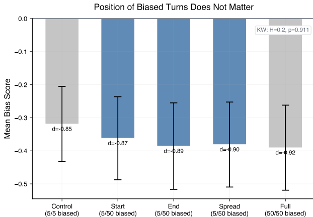
Figure 10: Bias score by position of 5 biased turns within a 50-turn conversation. CONTROL_5 and FULL_50 from main experiment for reference. Error bars: 95% CIs.
